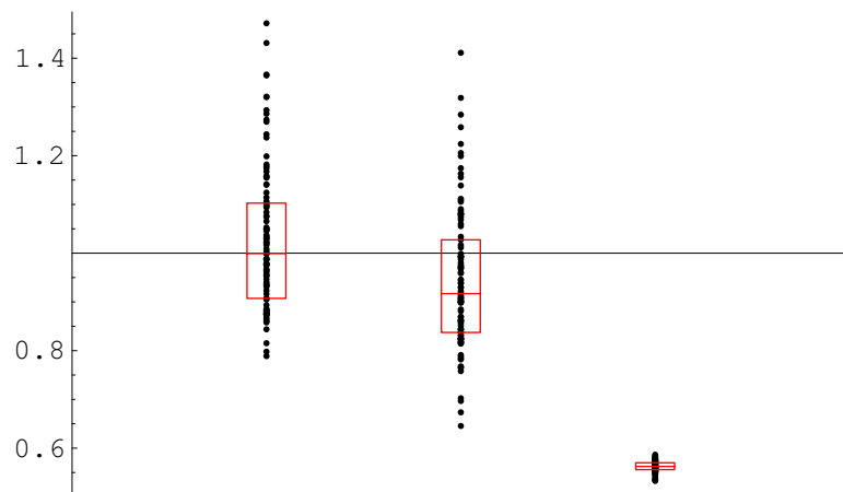
Figure 3: \kappa/\sigma = 2/3
