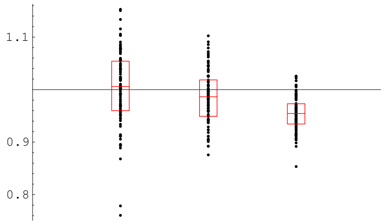
Figure 6: \kappa/\sigma = 2
