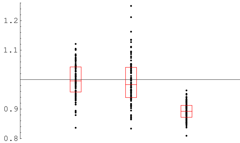
Figure 5: \kappa/\sigma = 3/2
