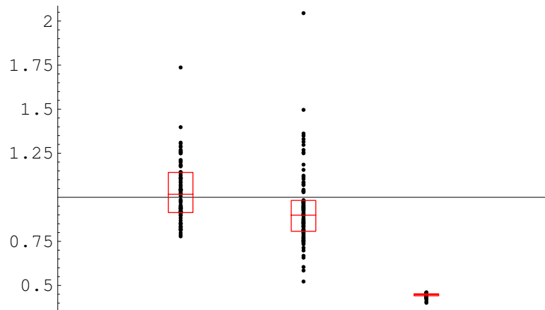
Figure 2: \kappa/\sigma = 1/2
