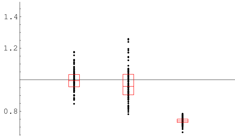
Figure 4: \kappa/\sigma = 1
