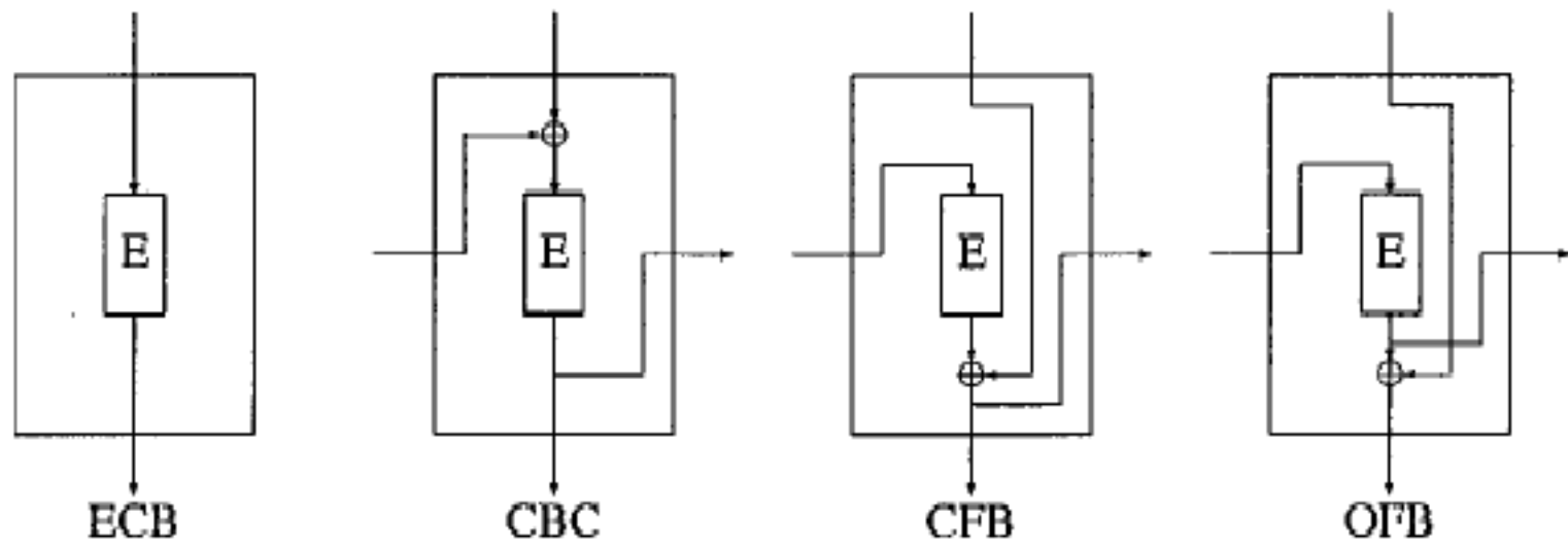
Fig. 1. DES modes of operation.
